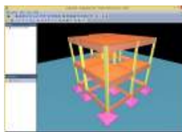
Figura 2: Software TQS
